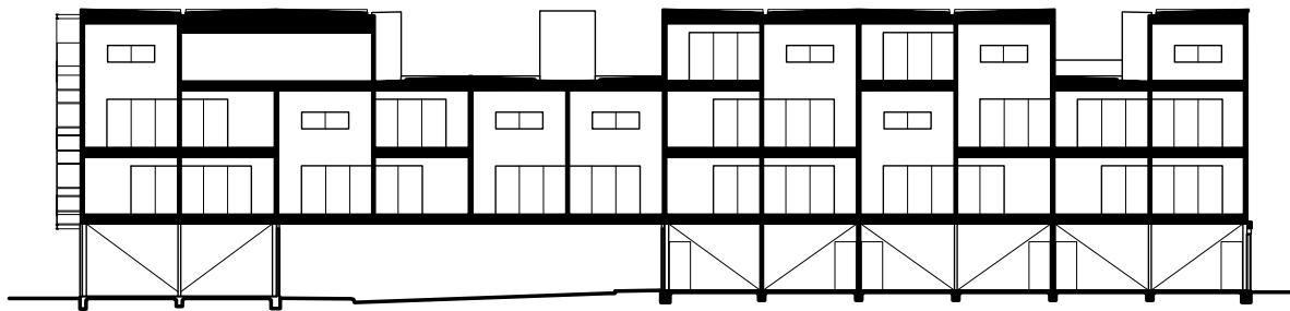
NORTH/SOUTH SECTION
