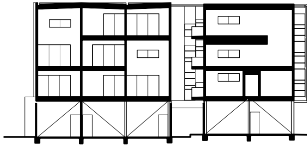
WEST/EAST SECTION
