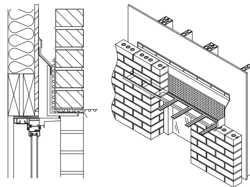
VENEER WINDOW HEADS
